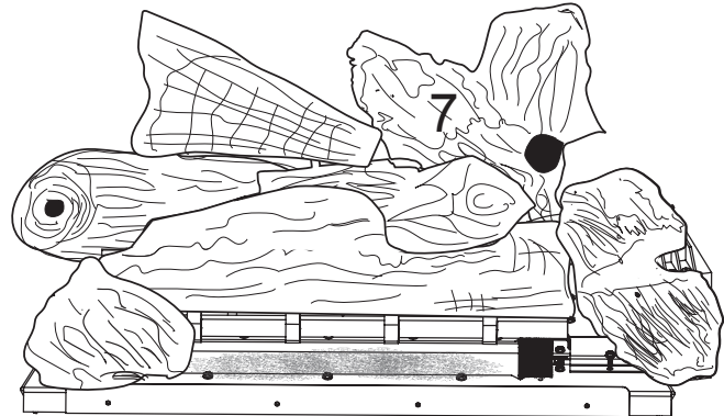
Figure 5.17 - Log #7 Placement
